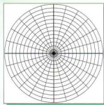
Concentric circles on 1 3/4" (44.45 mm) centers. Lines to circumference are 15 degrees apart. Outside circle 45" (1143 mm) diameter. 1/32" (.79 mm) thick lines. 5/32" (3.72 mm) X and Y line thickness.
