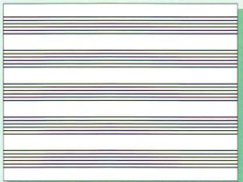
Five 1/16" (1.58 mm) lines per section. 1" (25.4 mm) line spacing, 5" (127 mm) between sections. 4" (101.6 mm) border, top and bottom.
